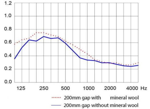
Absorption according to EN ISO 354
